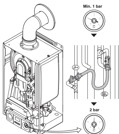
Fig.10 Water pressure
